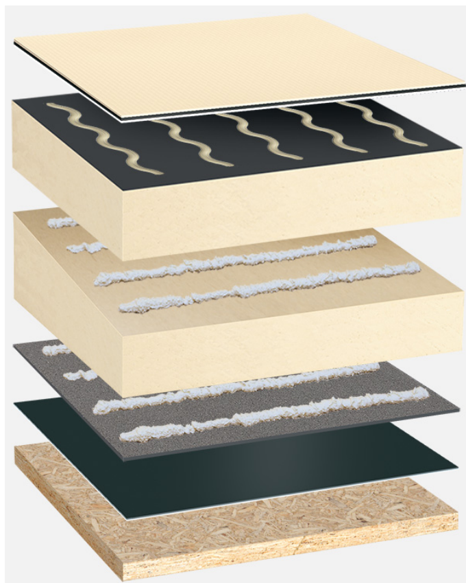
Sustav: HP_PIR-TG_PIR-FA_TV_01
